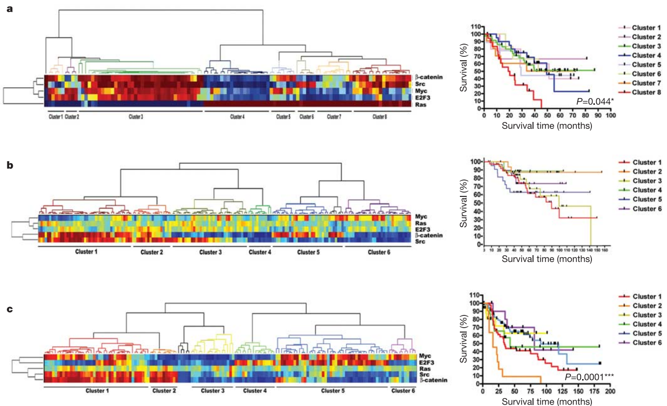
Figure 3 | Patterns of pathway deregulation in human cancers. a , Hierarchical clustering of predictions of pathway deregulation in samples of human lung tumours (left panel). Prediction of Ras, Myc, E2F3, \beta -catenin and Src pathway status for each tumour sample was independently determined using supervised binary regression analysis, as described. Red indicates high probability of pathway activation, with blue indicating a low probability. Patterns in the tumour pathway predictions were identified by
